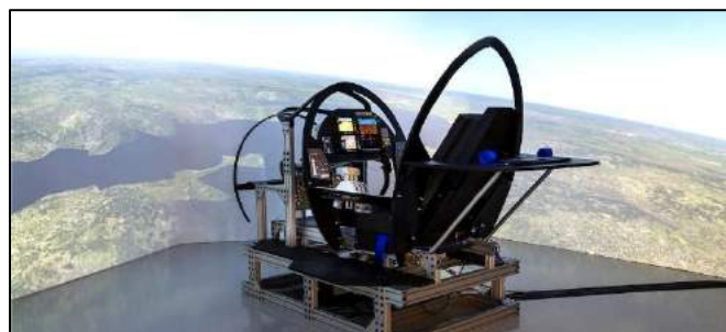
Figure 8 - Portable Flight Simulator
